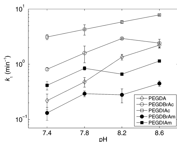
Figure 4. Rate constants for thiol consumption by PEG cross-linkers, including PEGDA as a control.
